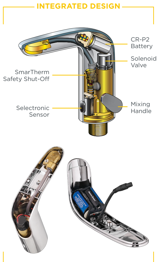
Remove Cover Screw to Change Battery or Service Solenoid Valve
